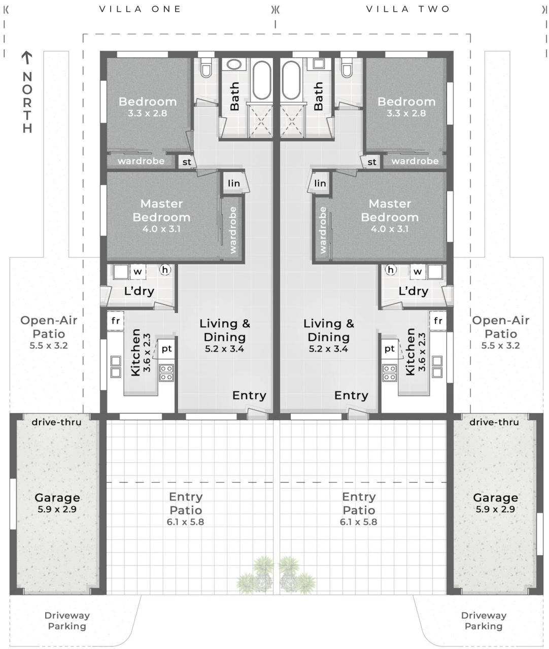
:: FLOOR PLAN
