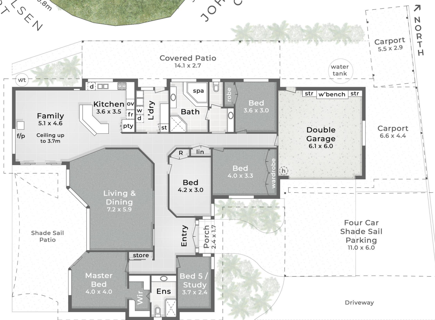
:: FLOOR PLAN 2.6m Ceiling
