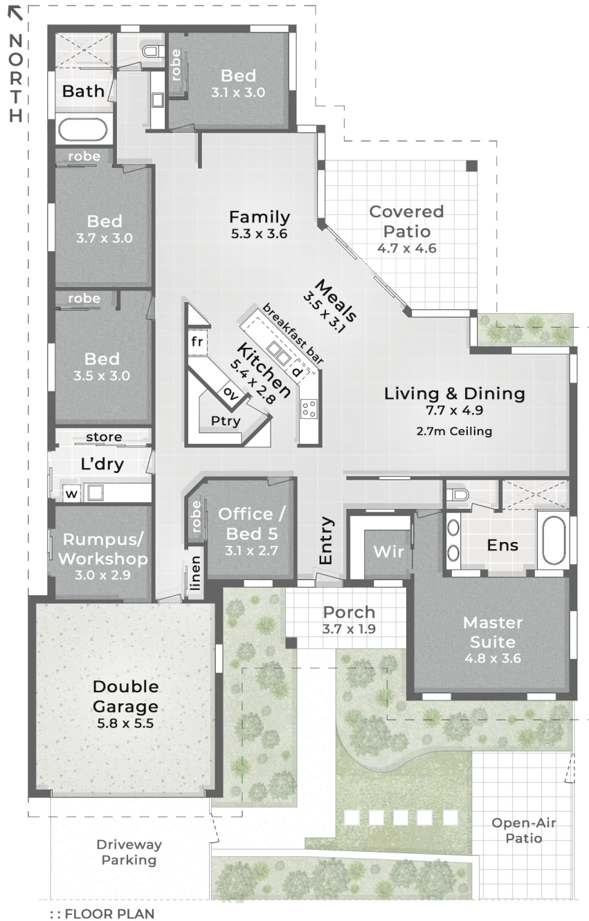
:: FLOOR PLAN
